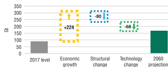
Figure 39: Global material use in 2017 and 2060, and impact of structural and technology change
